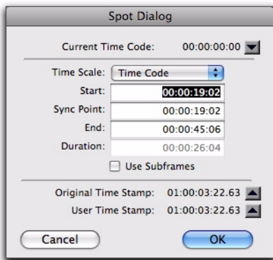
Spot dialog
