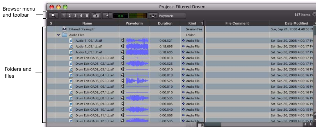
Figure 1. Project browser
